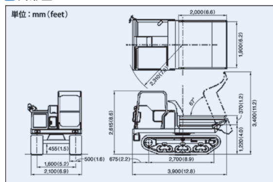
MST-700VDR
